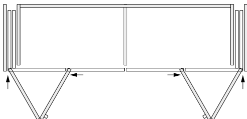
Hawa Folding Concepta III 20 Pull, left/right
