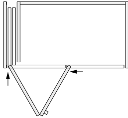
Hawa Folding Concepta III 20 Pull, left
